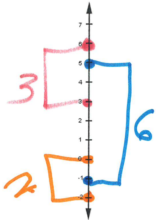
Figure 3 - Vertical Number Line
